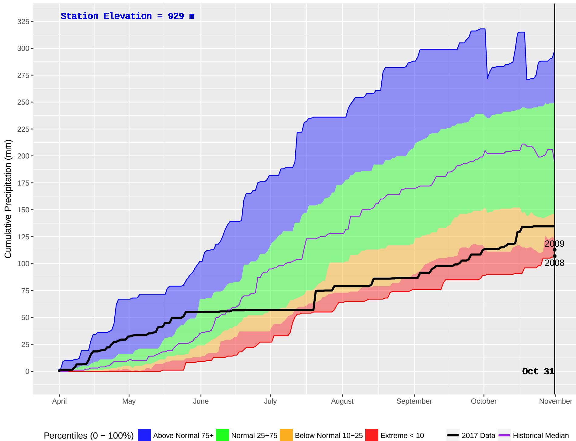
RISKE CREEK (210) : Historical (1980–2016) and Current (2017) Noon Cumulative Precipitation
