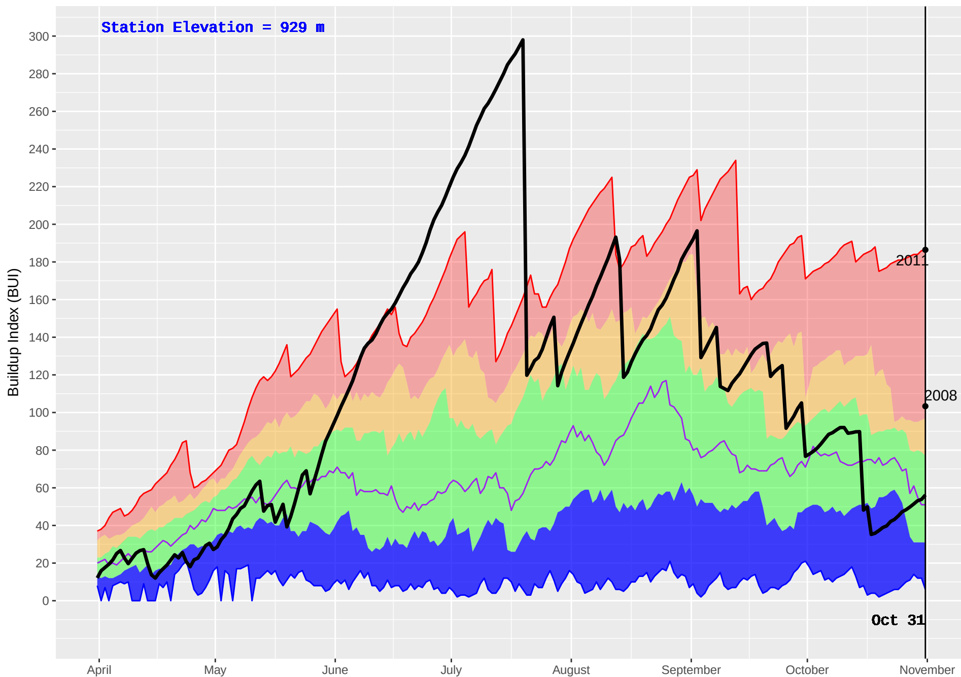
RISKE CREEK (210) : Historical (1980–2016) and Current (2017) Noon Buildup Index (BUI)
