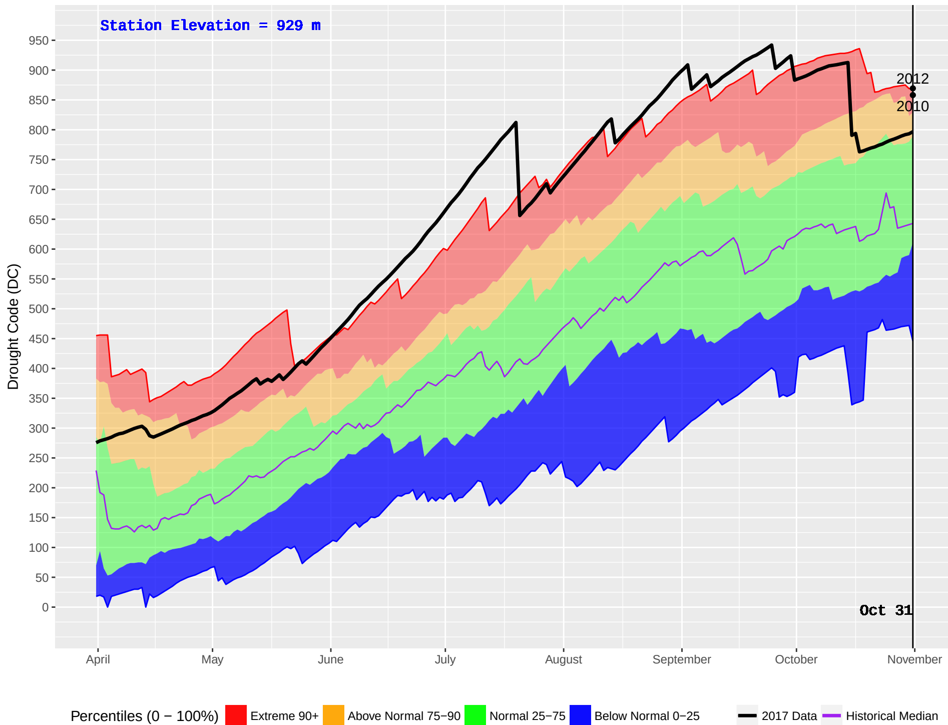
RISKE CREEK (210) : Historical (1980–2016) and Current (2017) Noon Drought Code (DC)
