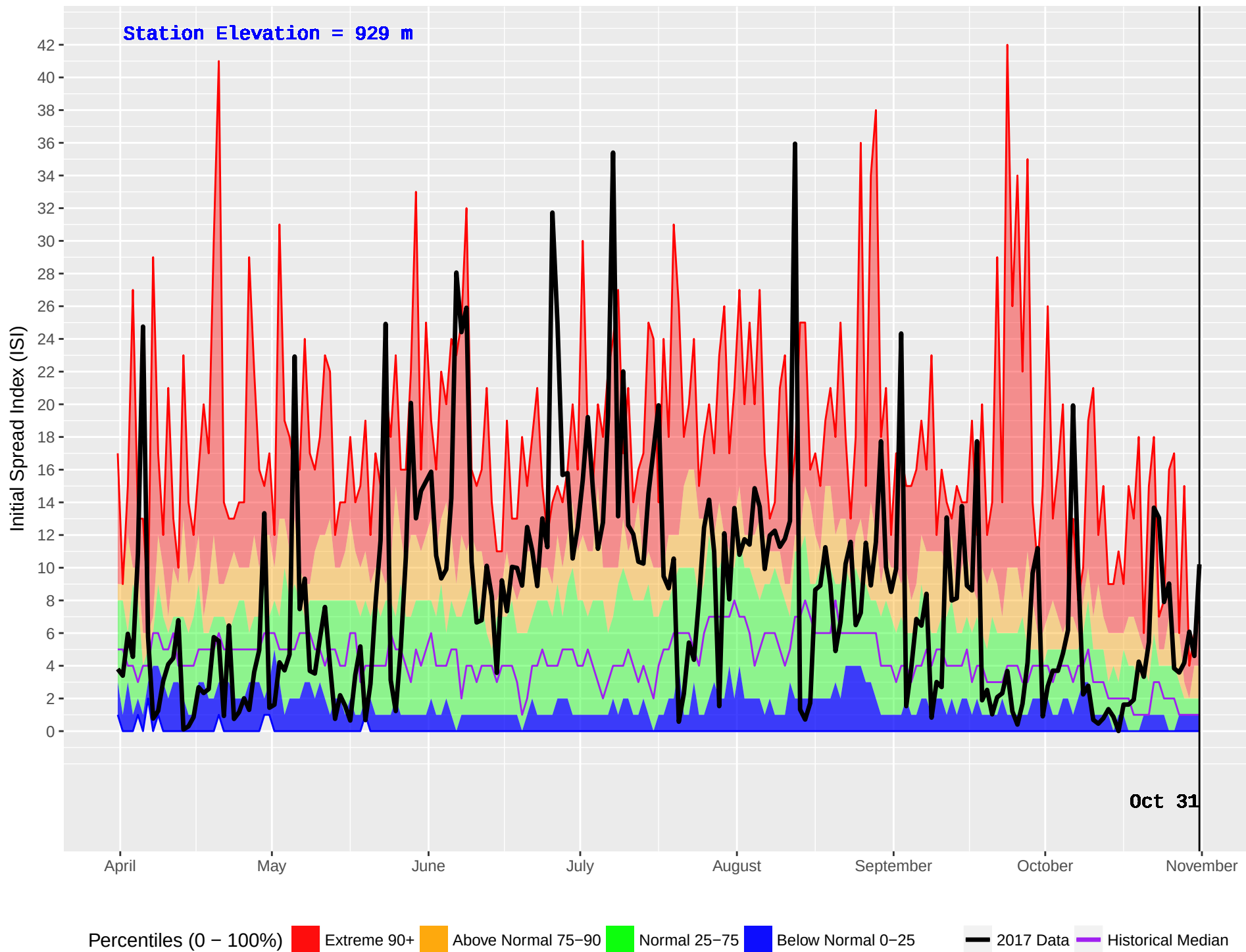
RISKE CREEK (210) : Historical (1980–2016) and Current (2017) Noon Initial Spread Index (ISI)
