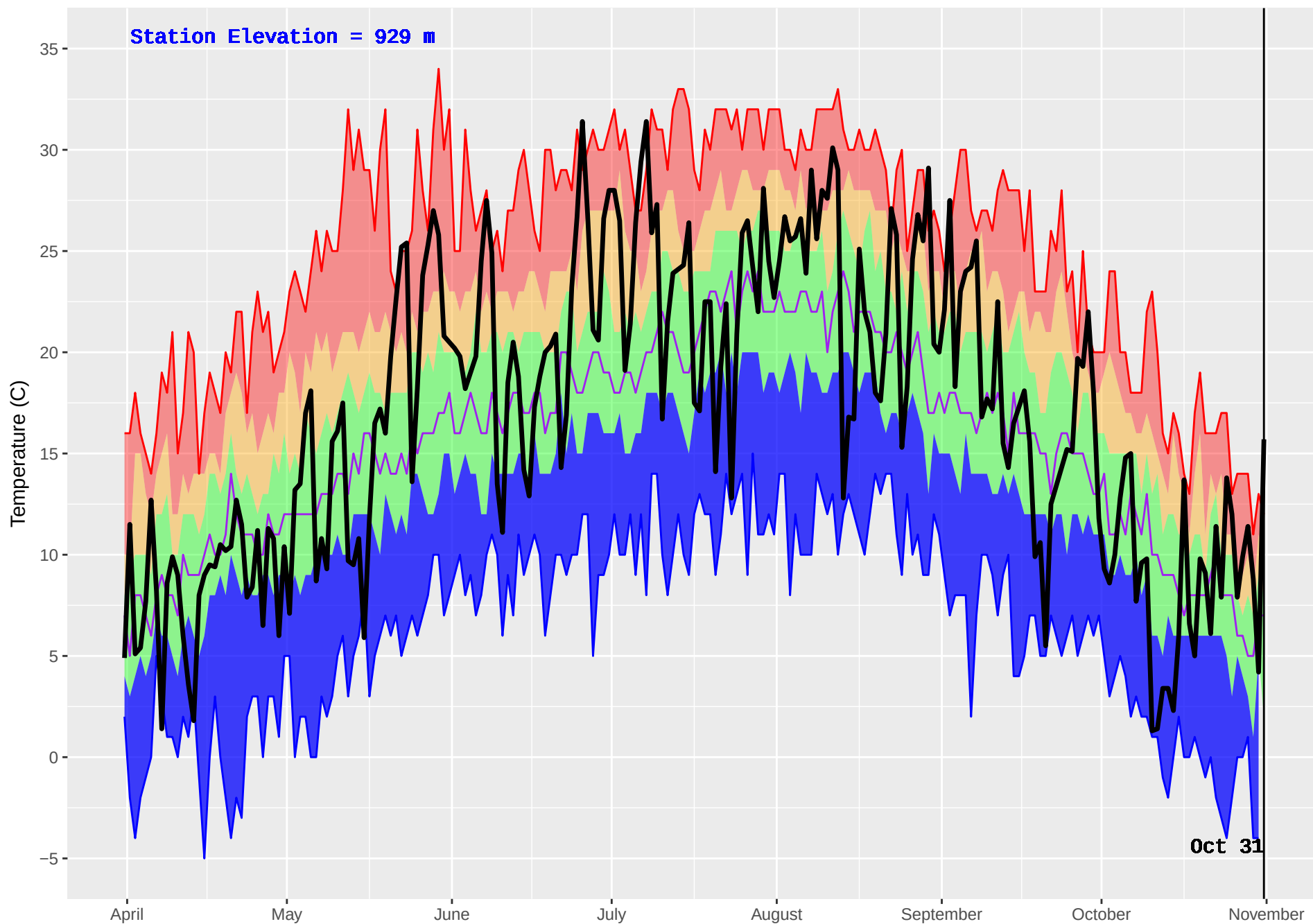
RISKE CREEK (210) : Historical (1980–2016) and Current (2017) Noon Temperature
