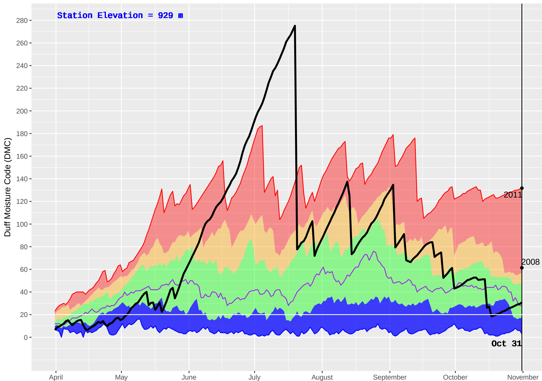
RISKE CREEK (210) : Historical (1980–2016) and Current (2017) Noon Duff Moisture Code (DMC)
