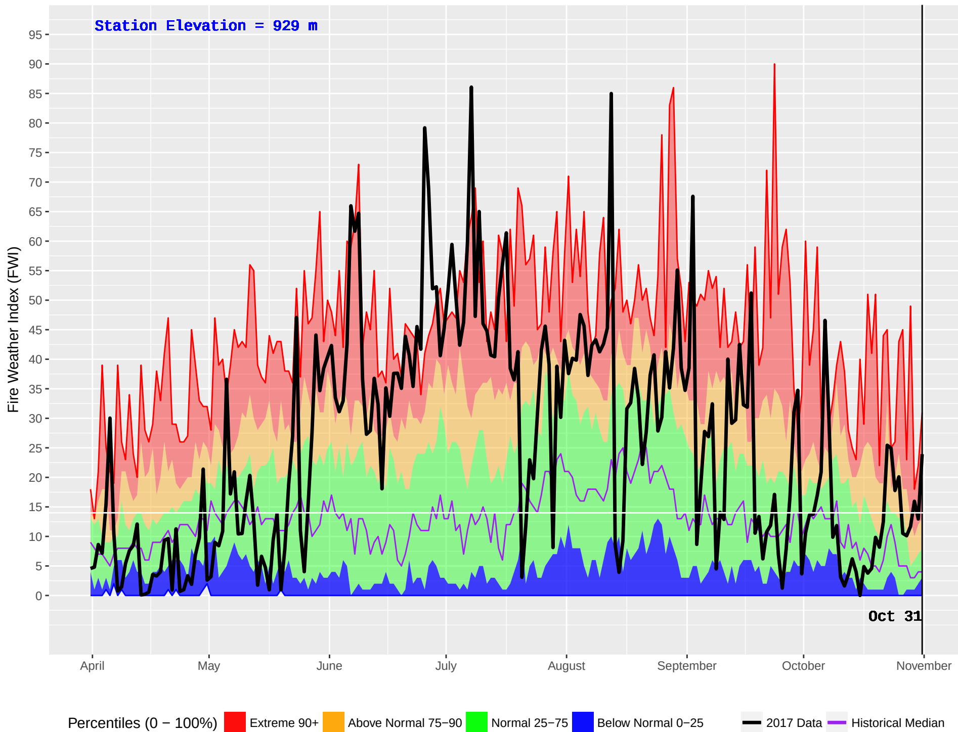
RISKE CREEK (210) : Historical (1980–2016) and Current (2017) Noon Fire Weather Index (FWI)
