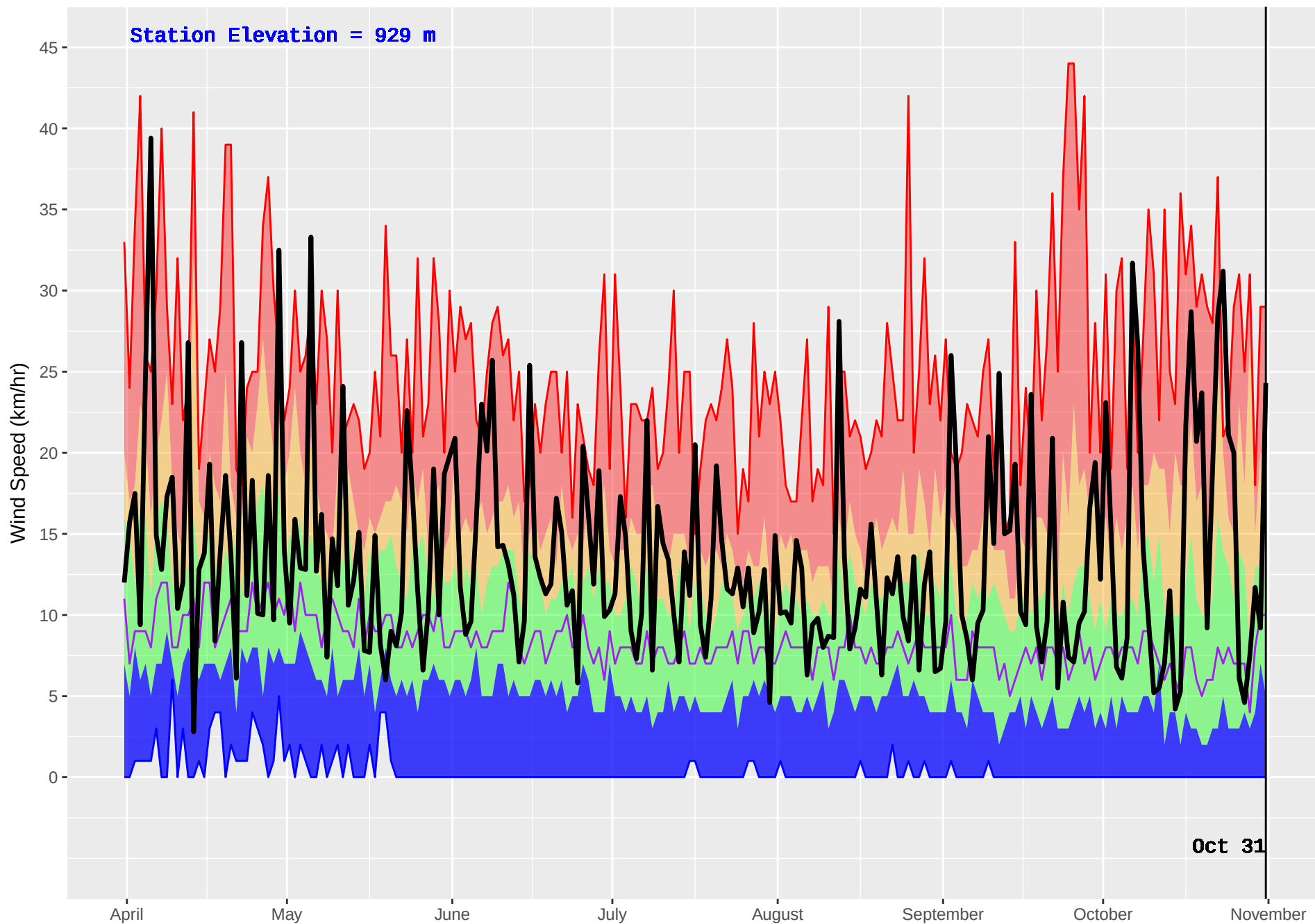
RISKE CREEK (210) : Historical (1980–2016) and Current (2017) Noon Wind Speed
